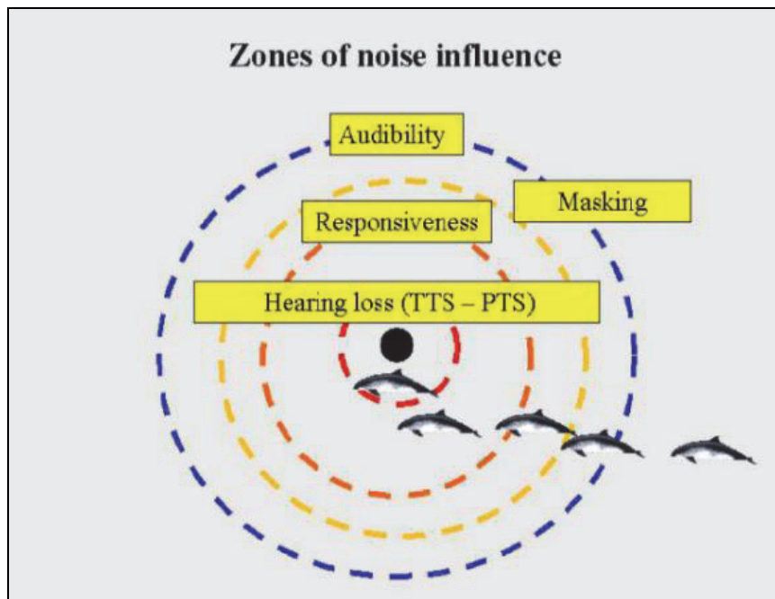
Figure 46: Zones of noise influence (after Richardson et al., 1995)
