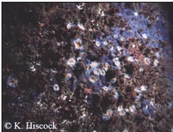
Sea anemones ( Actiniaria ), overlapping ascidians ( Ascidacea ), sponges ( Porifera ) and algae characteristics on intermediate depth & offshore structures
