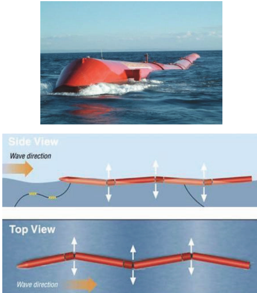
Figure 22: The "PELAMIS" system Source: energiebleue.e-monsite.com
