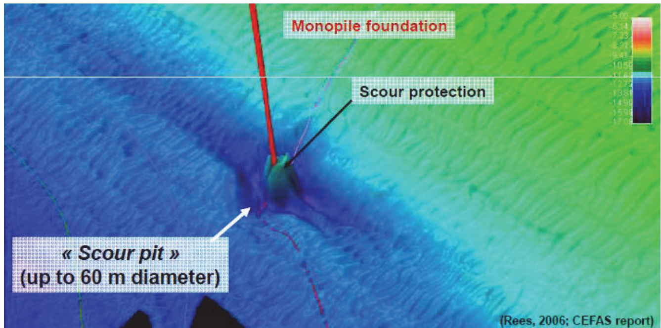
Figure 34: Leveling around a monopile Source: Rees, 2006
