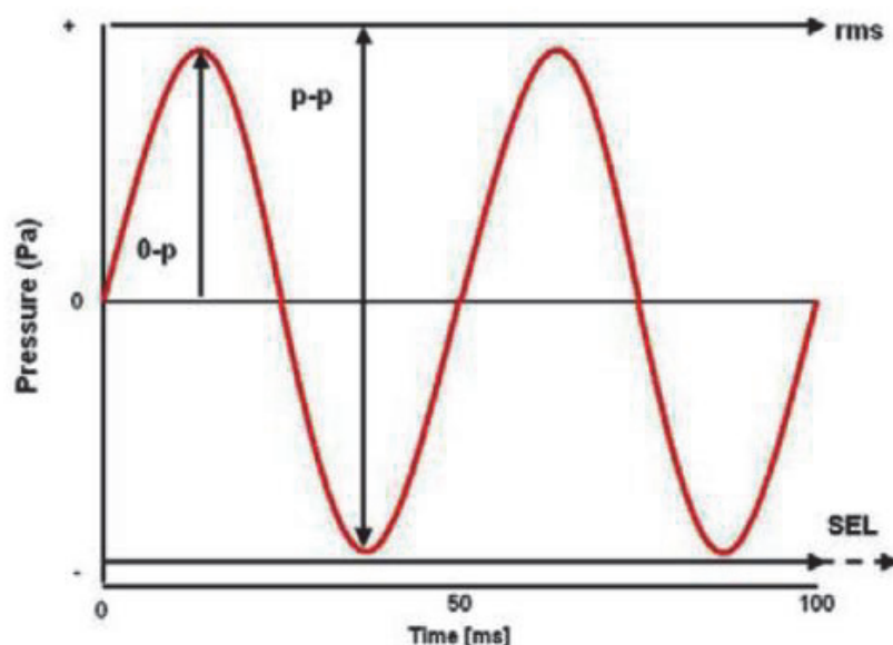
Figure 44: A simple sinusoidal waveform describing different units of measurement of sound Source: Thomsen et al., (2006)
