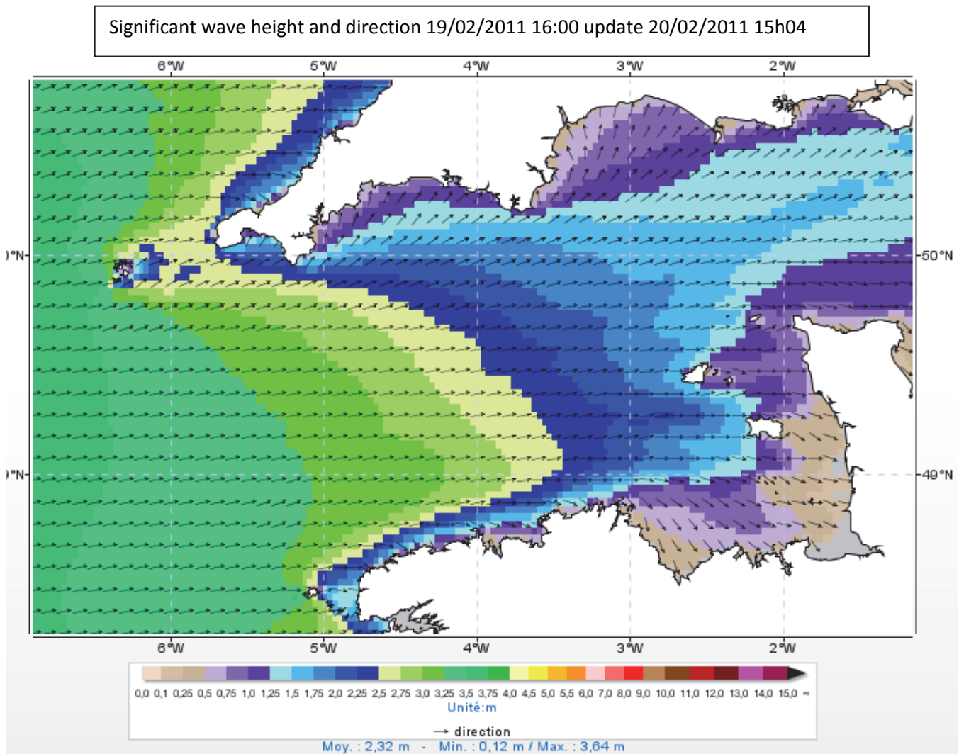
Figure 19: Significant wave height, 19 February 2011 in accordance with the Previmer model, between Cornwall UK and Finistère Source : previmer.com
